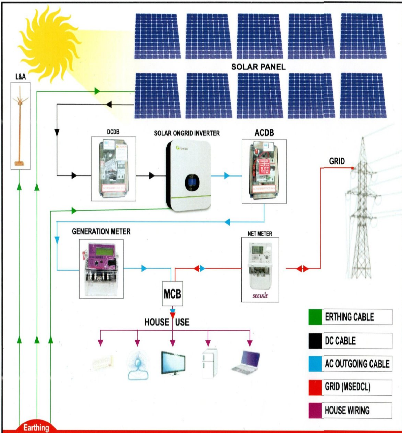
Single Line Diagram of Solar Power Plant
